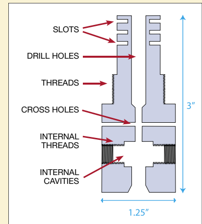
The sPINner deburrs external and internal part geometry.
